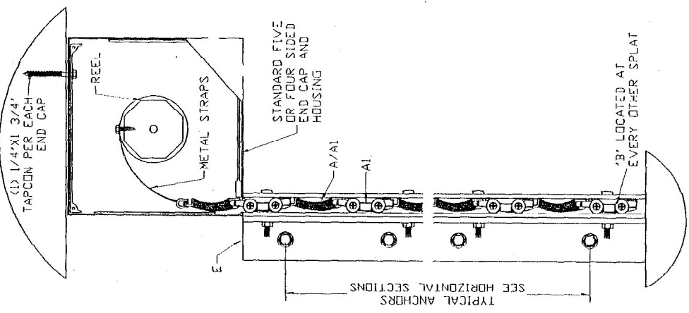
SECTION CC/DD INSET MOUNT
