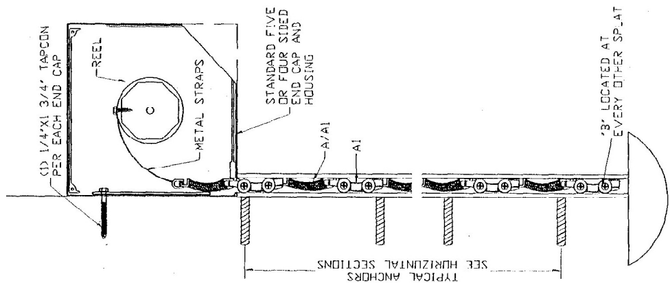
SECTION CC/DD WALL SECTION
